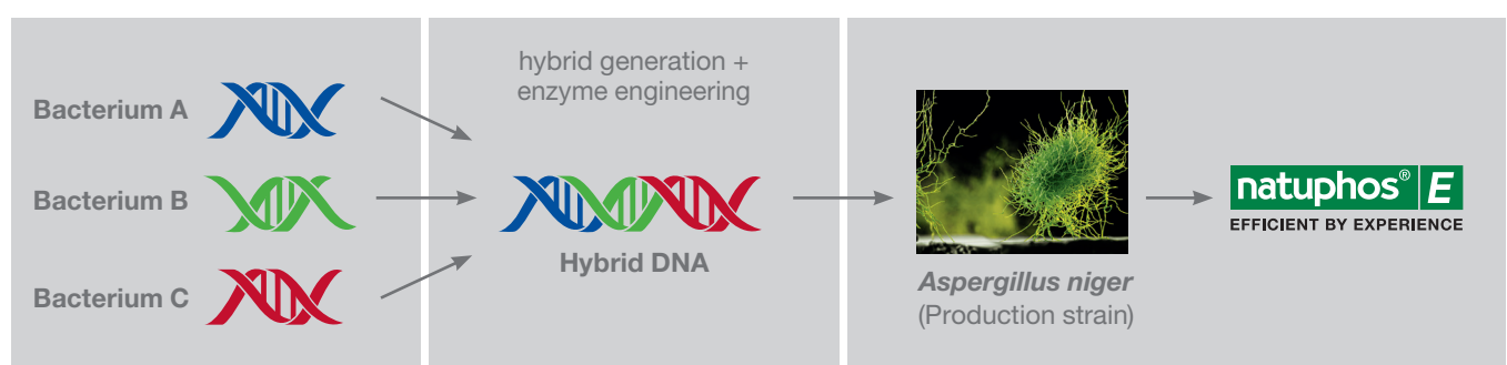
FIGURE 1: NOVEL HYBRID 6-PHYTASE
